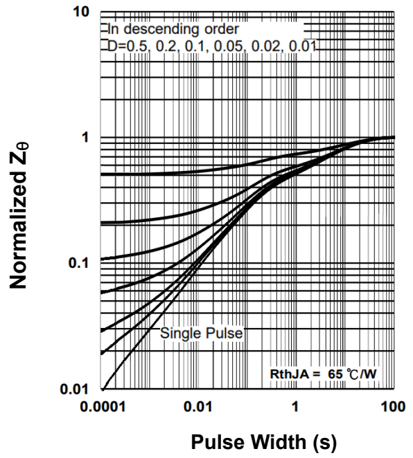
FIG.10 Normalized Transient Impedance
