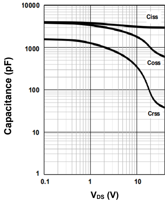
FIG.8 Capacitance Characteristics
