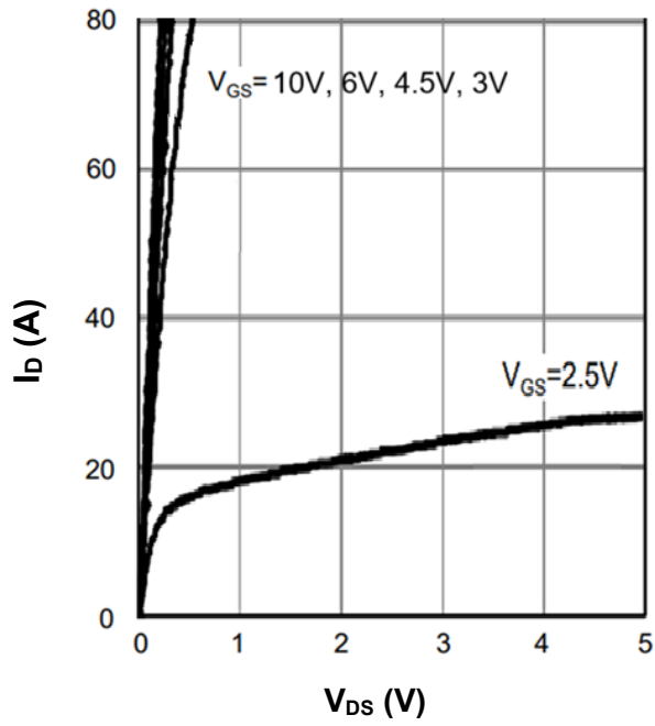
FIG.1 Output Characteristics
