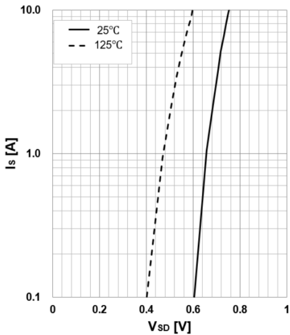
FIG.11 Body-Diode Characteristics
