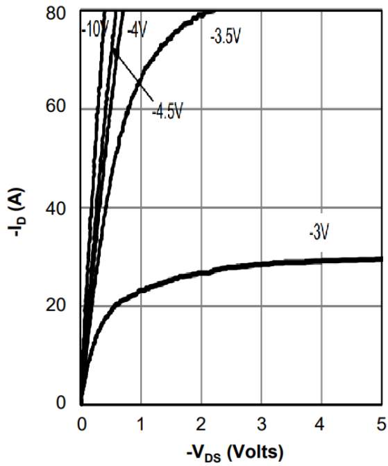
FIG.1 Output Characteristics
