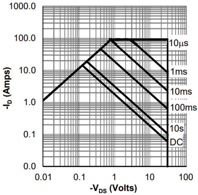
FIG.9 Maximum Safe Operation Area
