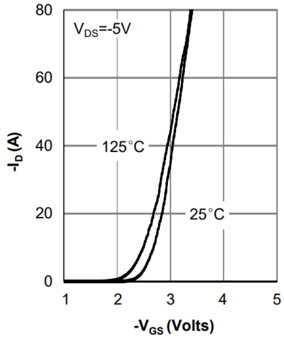
FIG.2 Transfer Characteristics
