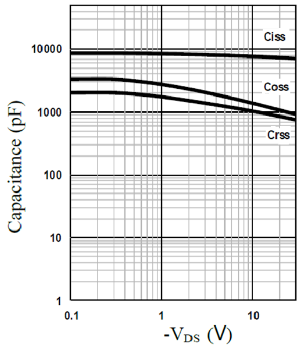
FIG.8 Capacitance Characteristics
