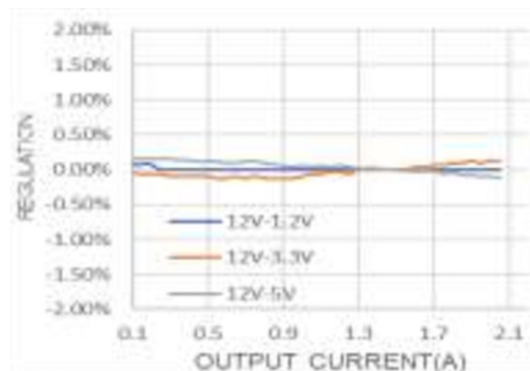
FIG 2. Load Regulation
