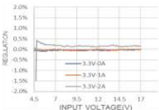
FIG 3. Line Regulation
