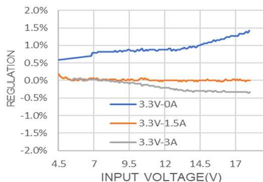
FIG 3. Line Regulation
