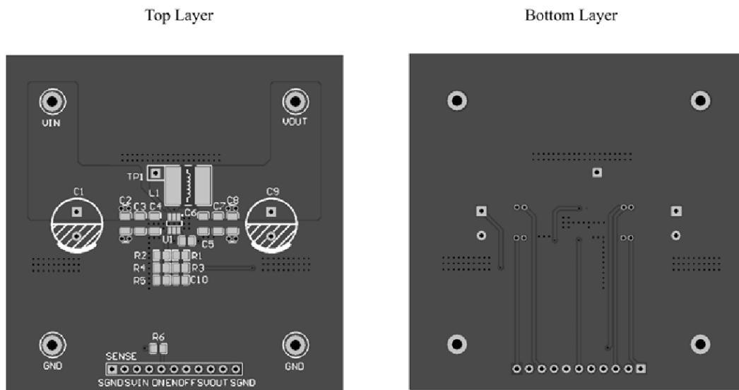
Sample Board Layout
