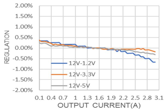
FIG 2. Load Regulation
