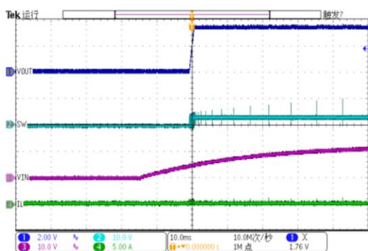
FIG 15. Power Up at No Load
