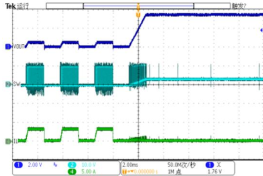
FIG 10. Short Circuit Recovery
