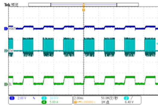
FIG 8. Output Short
