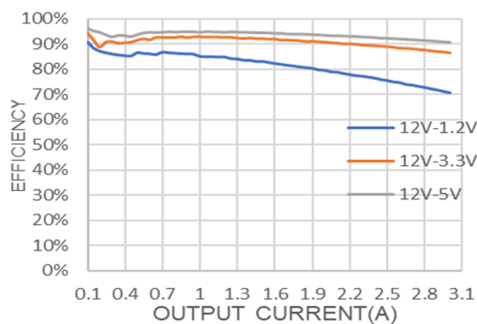
FIG 1. Efficiency vs Load Current
