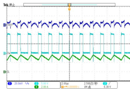
FIG 6. Output Ripple Voltage
